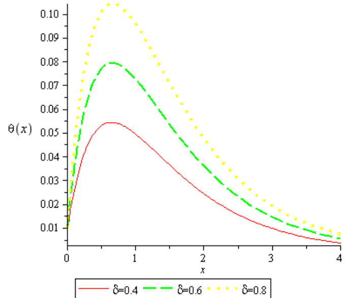
Figure 1: Plots of \theta(x) against x for equation (25) for different values of \delta and \alpha = 1, b = 1, \theta_b = 0.01, \epsilon = 0.01, e = 2.718, \nu_o = \nu_f = 1 .
