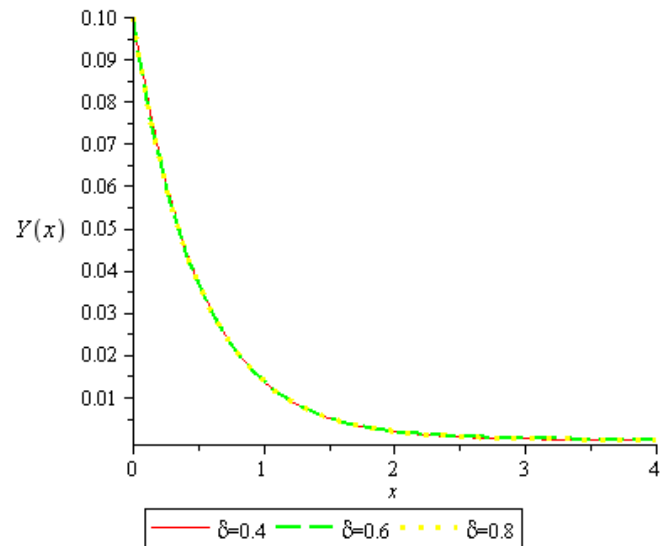
Figure 2: Plots of Y(x) against x for equations (24) and (25), for different values of \delta and \alpha = 1, b = 1, \theta_b = 0.01, \epsilon = 0.01, e = 2.718, \nu_o = \nu_f = 1 .
